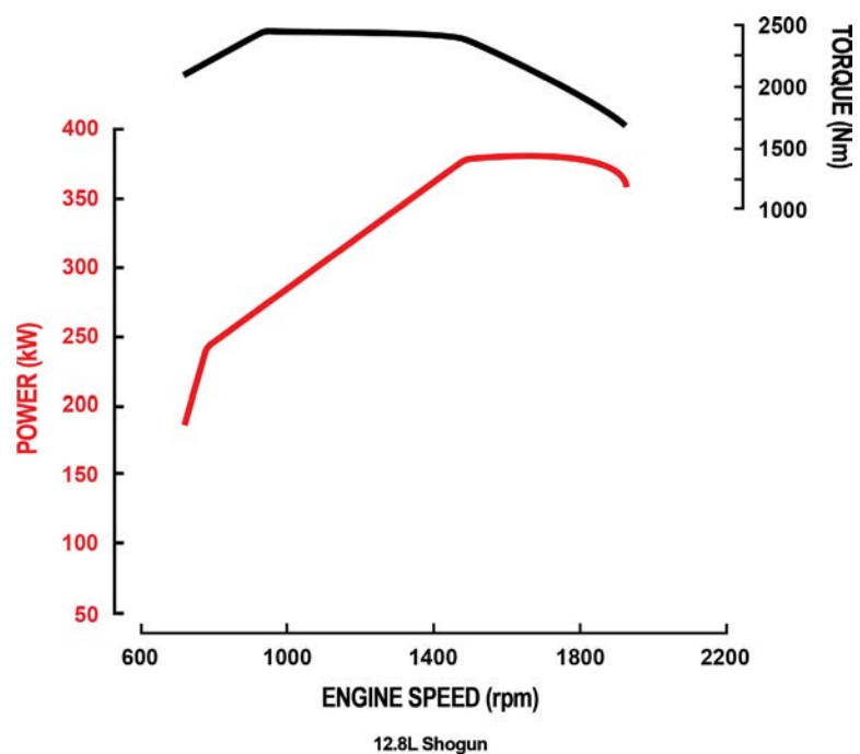
FUSO 6R30-T5 (390kW/2600Nm)
